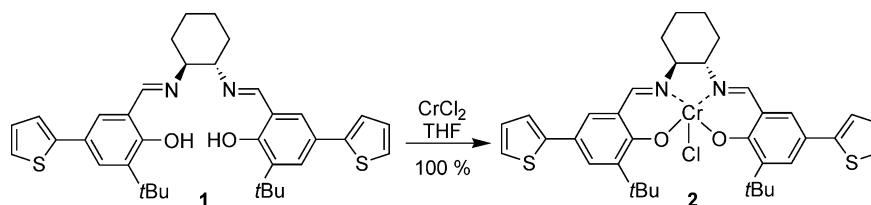
Scheme 1. Synthesis of chromium-thiophene-salen complex 2 .
