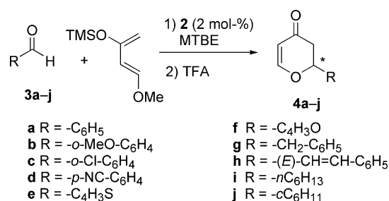
Scheme 3. HDA reaction of various aldehydes with Danishefsky's diene in the presence of chiral complex 2 .
