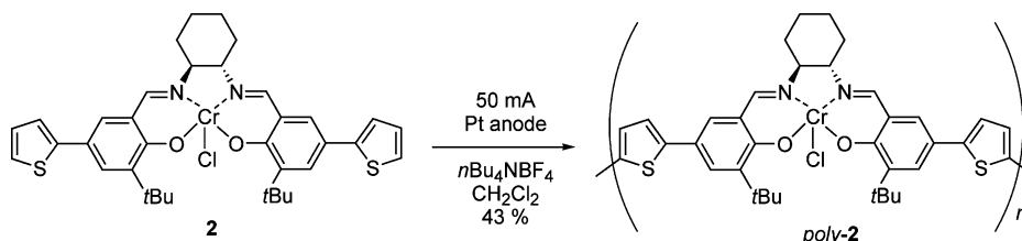
Scheme 2. Anodic polymerization of complex 2 in the synthesis of poly-2 .
