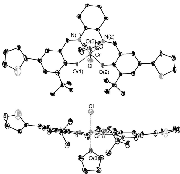
Figure 1. ORTEP drawing of complex 2 showing the atom labeling scheme. Ellipsoids are drawn at the 50% probability level. The THF solvate has been omitted. The hydrogen atoms have been omitted for the sake of clarity.
