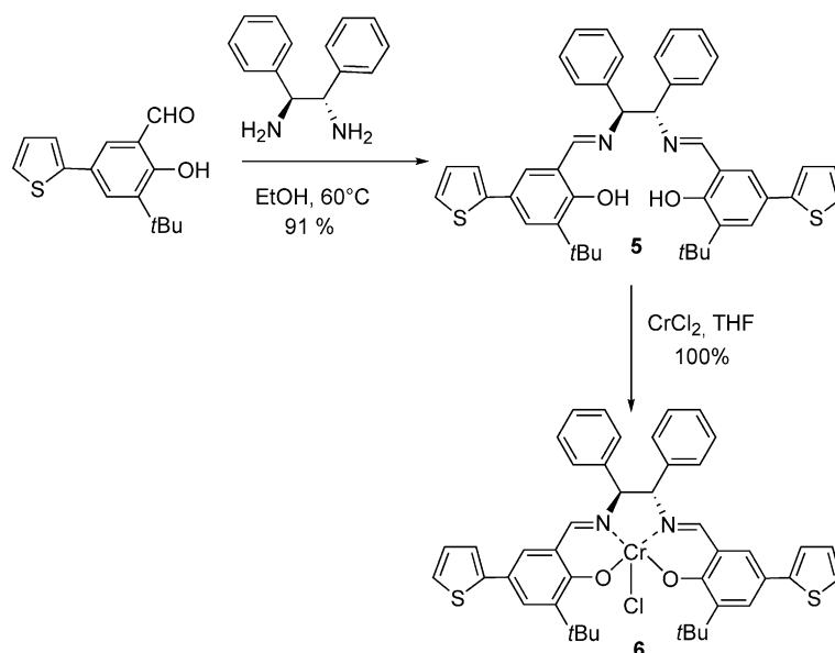
Scheme 4. Synthesis of the new chiral chromium complex 6 .
