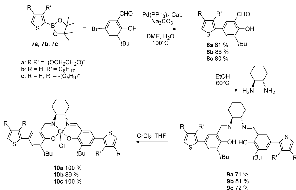
Scheme 5. Synthesis of the new chiral chromium complexes 10a–c .
