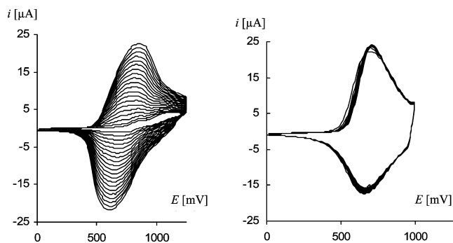
Figure 2. Left: anodic polymerization of chromium complex 2 (0.05 M) in \text{CH}_2\text{Cl}_2 with n\text{Bu}_4\text{NBF}_4 (0.1 M), v = 100 mV/s. Right: analysis of the polymer-coated electrode in \text{CH}_3\text{CN} with n\text{Bu}_4\text{NBF}_4 (0.1 M), v = 100 mV/s.
